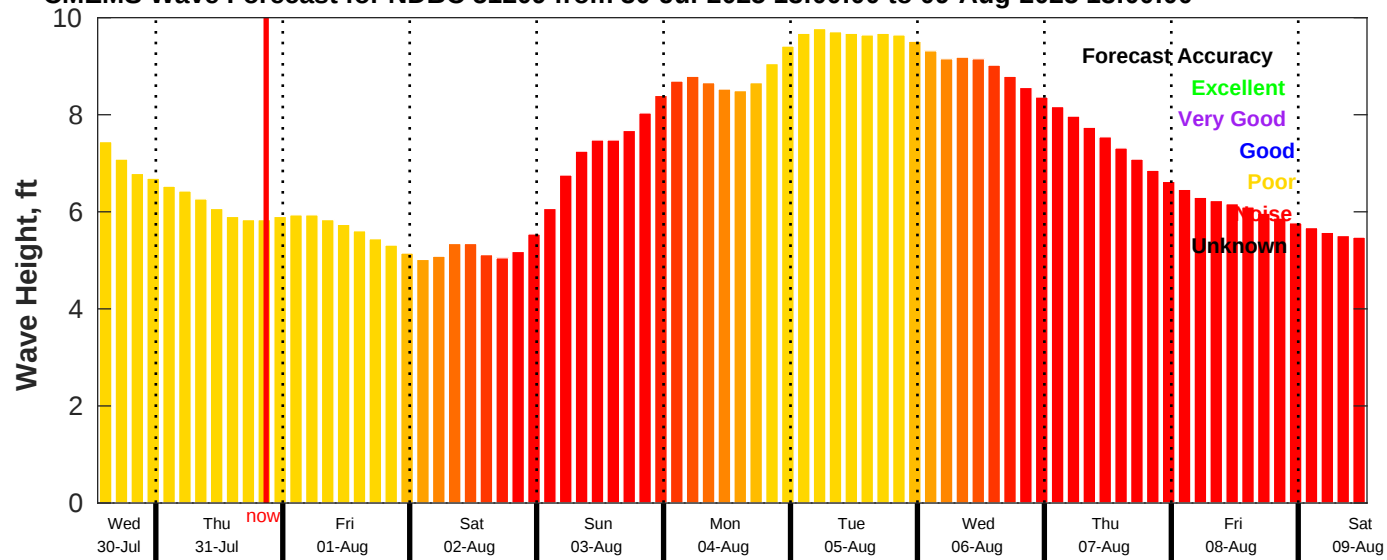
CMEMS Wave Forecast for NDBC 51209 from 30-Jul-2025 13:00:00 to 09-Aug-2025 13:00:00
