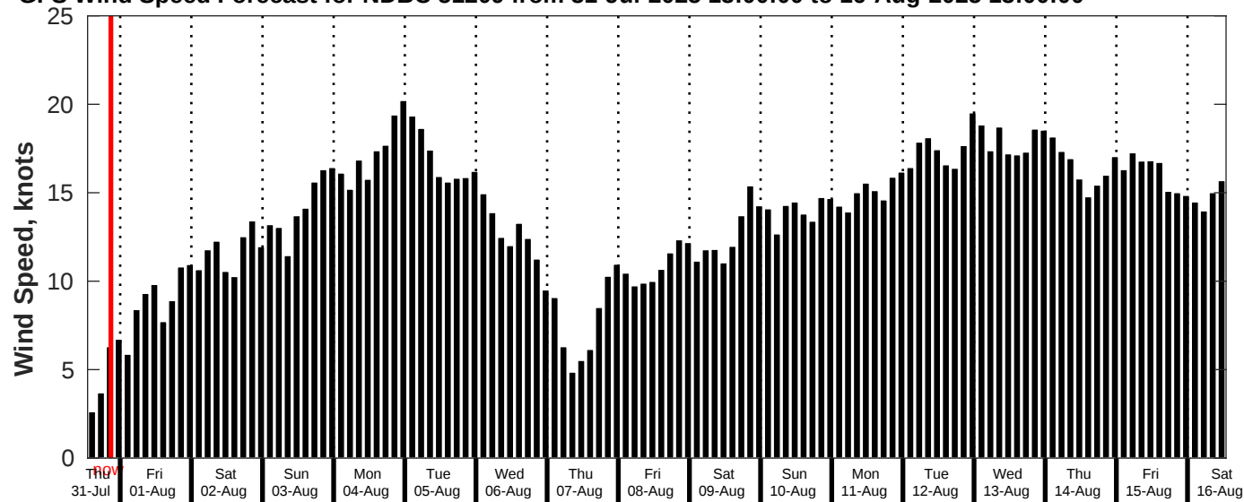
GFS Wind Speed Forecast for NDBC 51209 from 31-Jul-2025 13:00:00 to 16-Aug-2025 13:00:00
