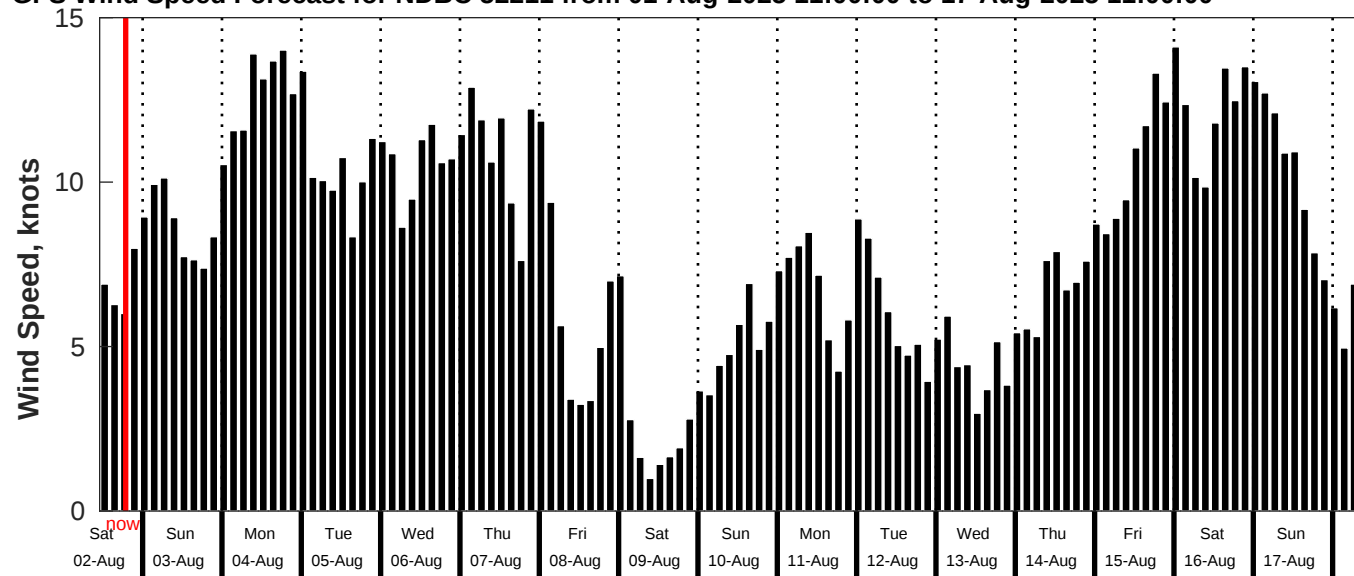
GFS Wind Speed Forecast for NDBC 52211 from 01-Aug-2025 11:00:00 to 17-Aug-2025 11:00:00
