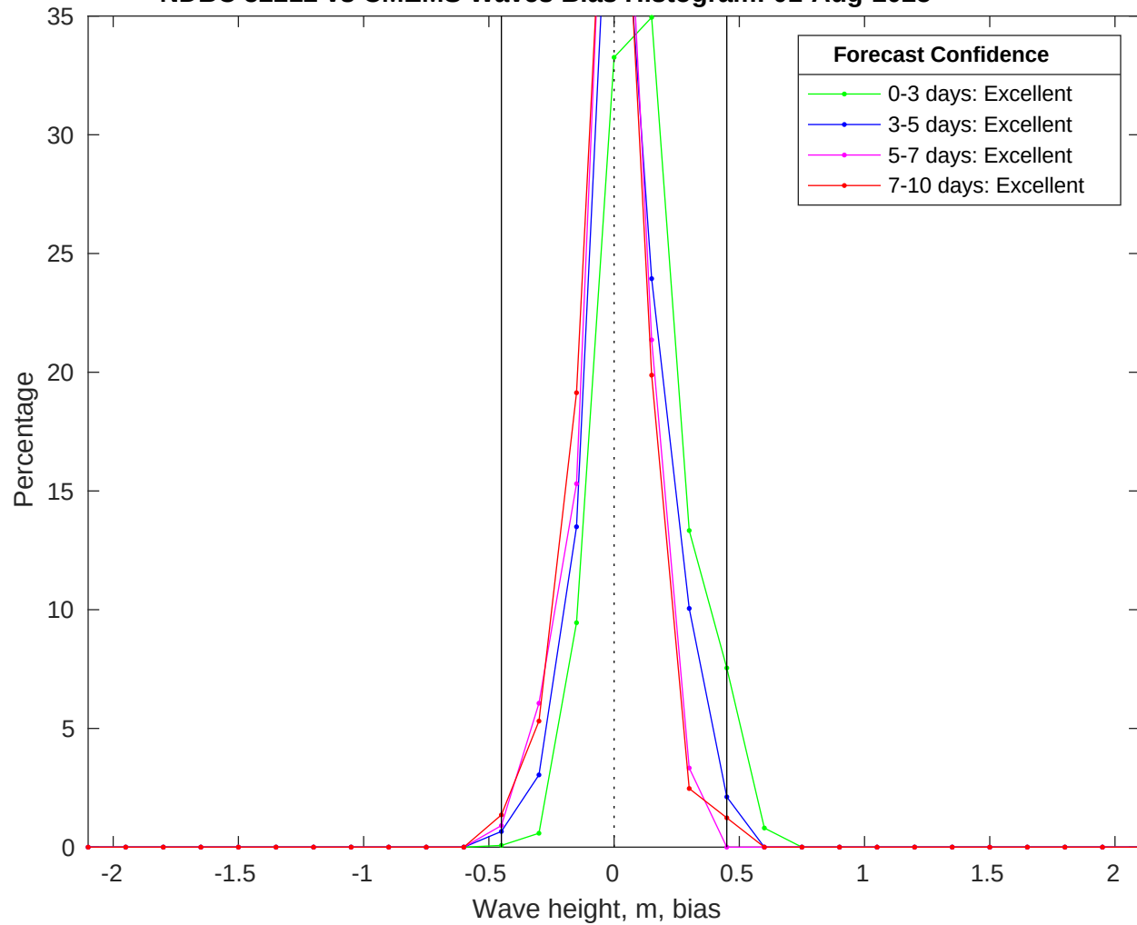
NDBC 52212 vs CMEMS Waves Bias Histogram: 01-Aug-2025
