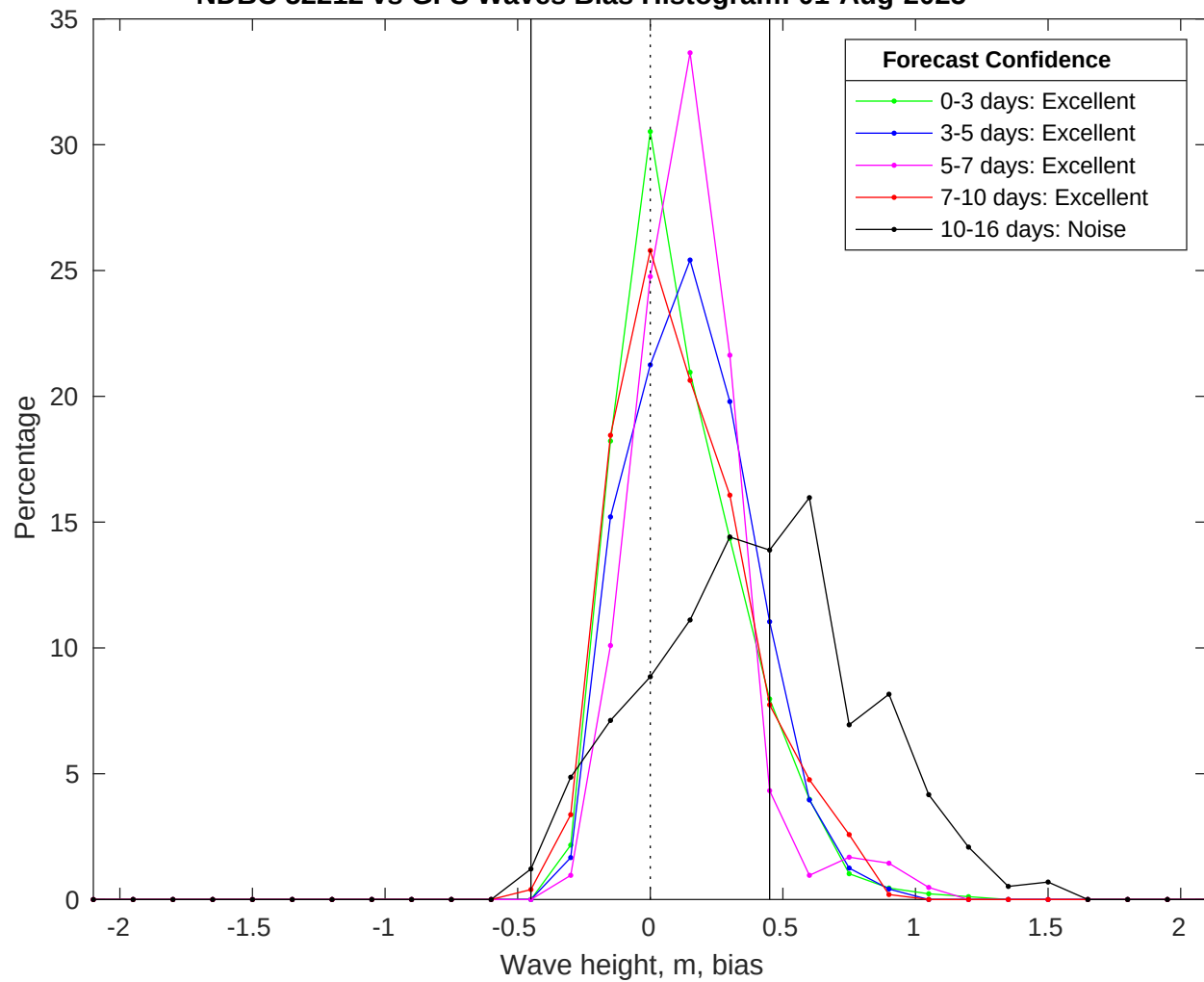
NDBC 52212 vs GFS Waves Bias Histogram: 01-Aug-2025
