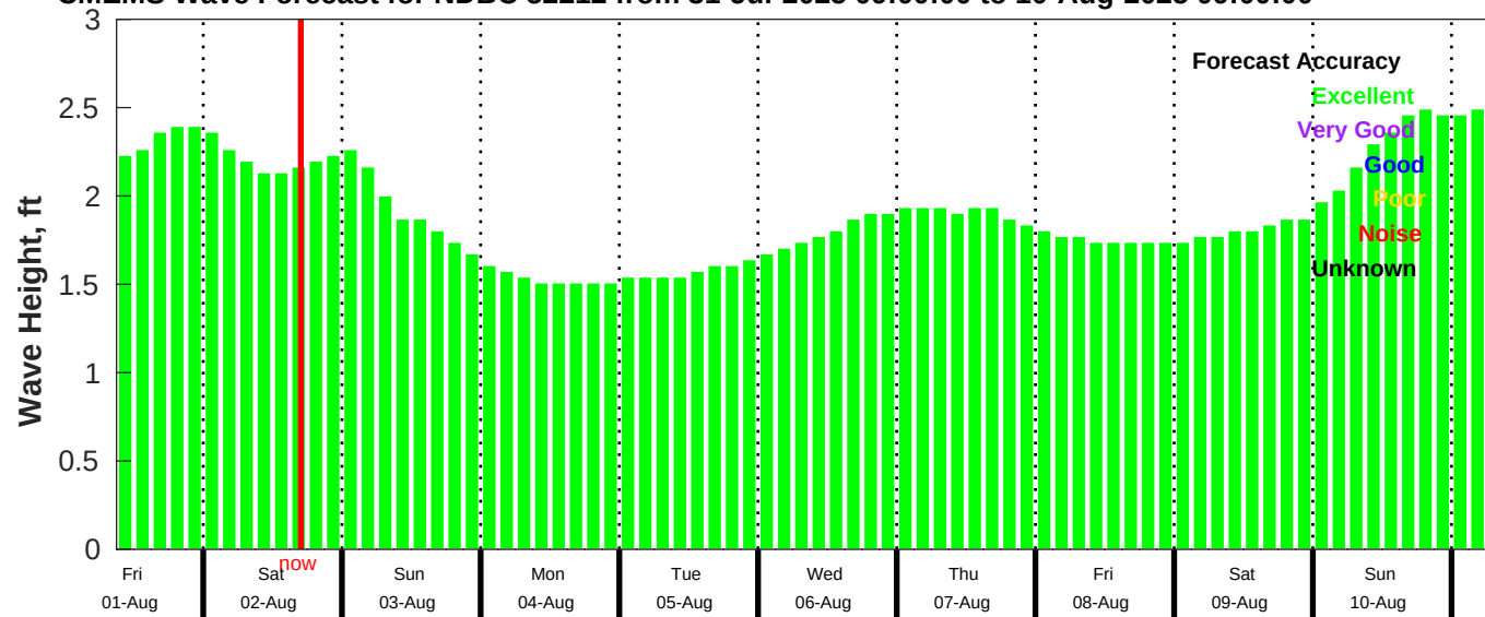
CMEMS Wave Forecast for NDBC 52212 from 31-Jul-2025 09:00:00 to 10-Aug-2025 09:00:00
