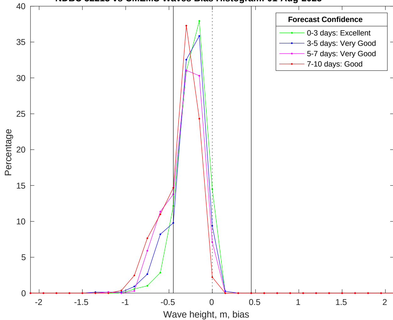
NDBC 52213 vs CMEMS Waves Bias Histogram: 01-Aug-2025
