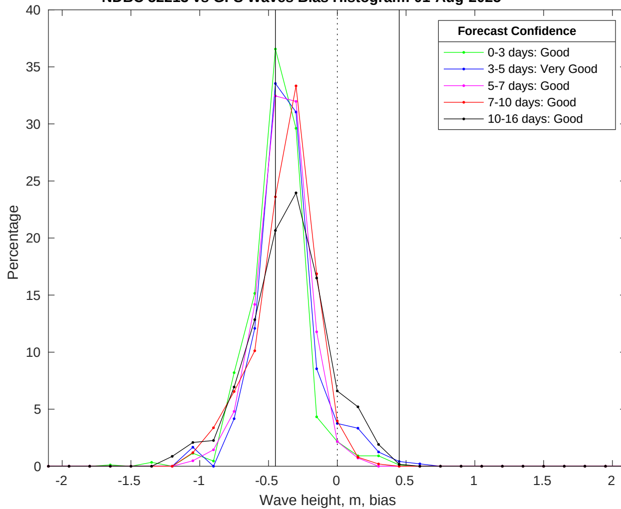
NDBC 52213 vs GFS Waves Bias Histogram: 01-Aug-2025
