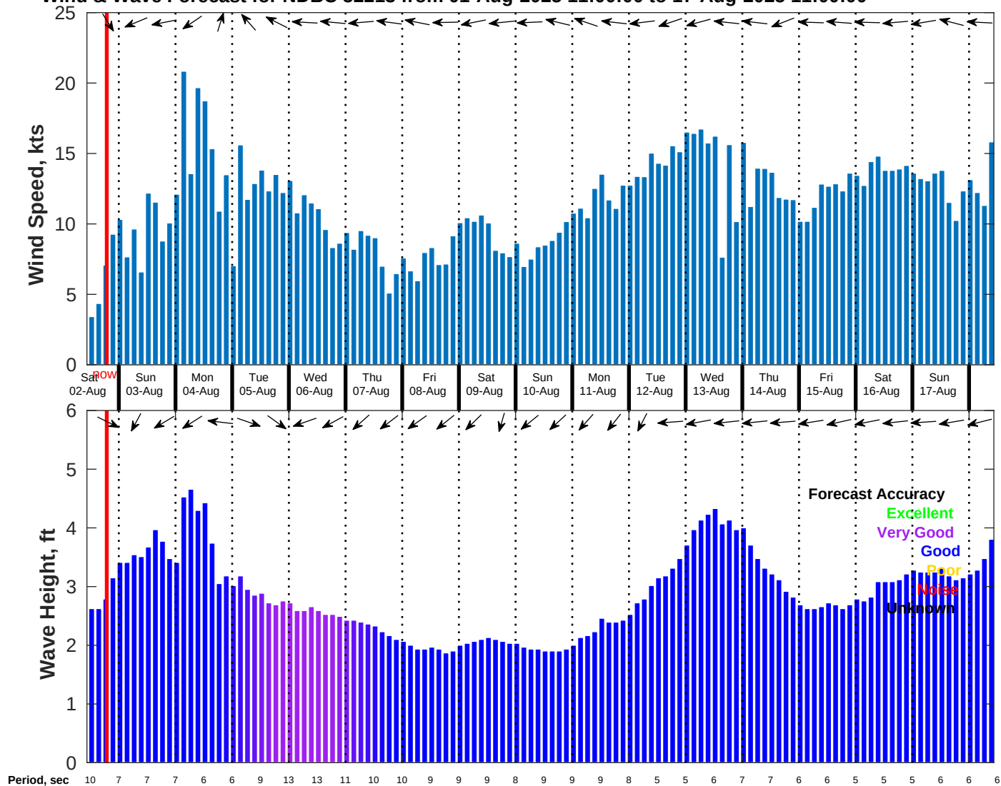
Wind & Wave Forecast for NDBC 52213 from 01-Aug-2025 11:00:00 to 17-Aug-2025 11:00:00
