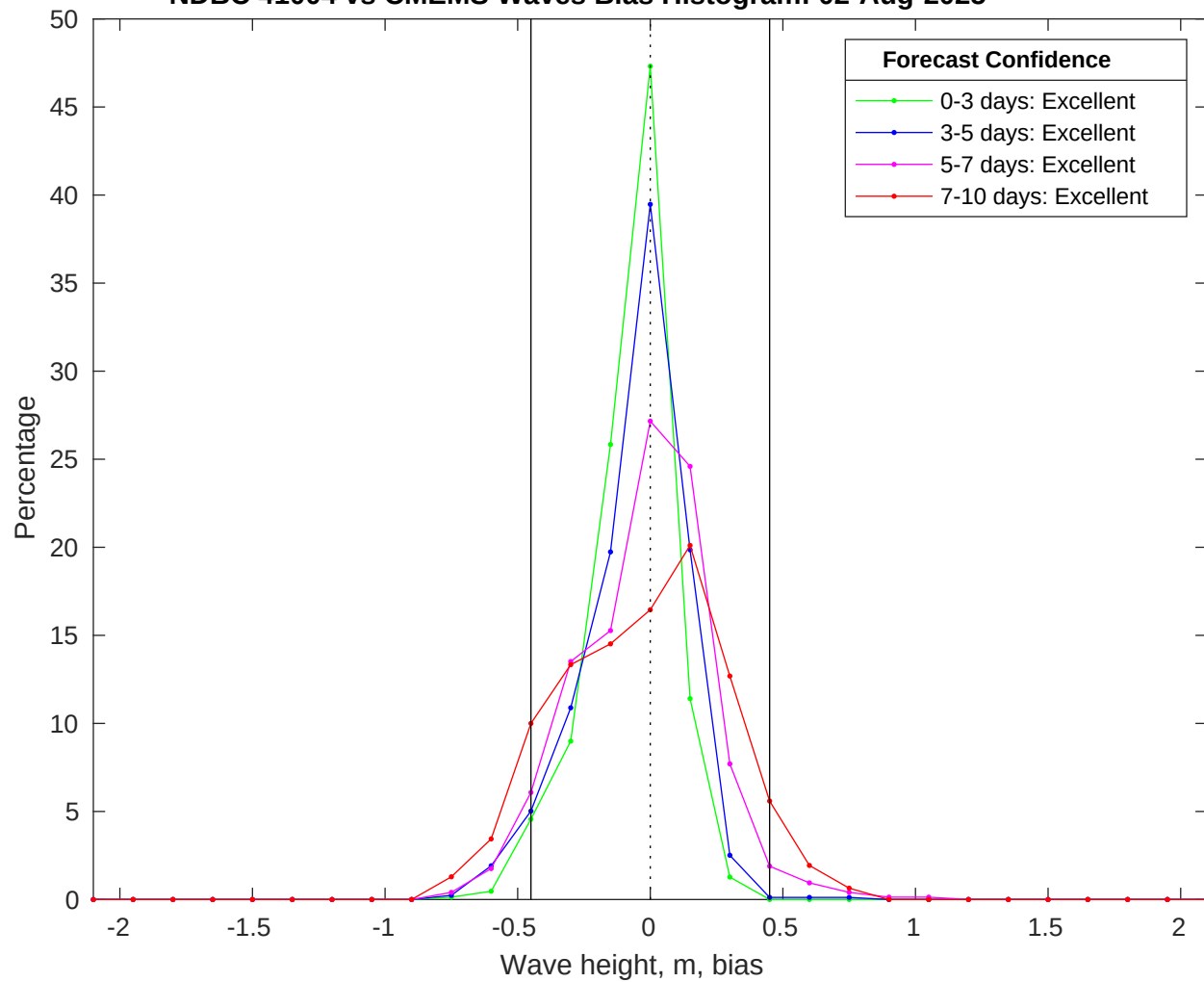
NDBC 41004 vs CMEMS Waves Bias Histogram: 02-Aug-2025
