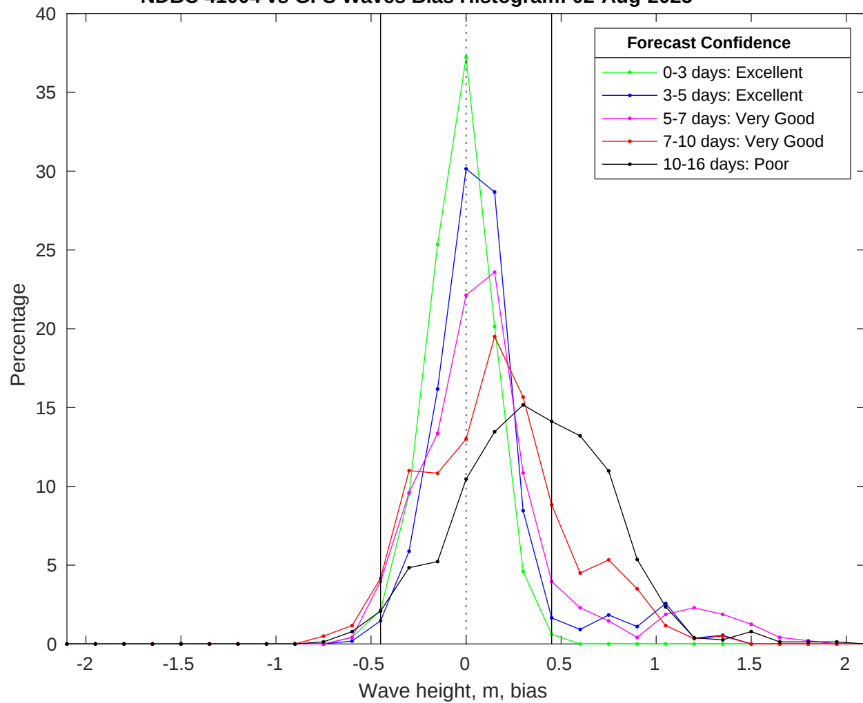
NDBC 41004 vs GFS Waves Bias Histogram: 02-Aug-2025
