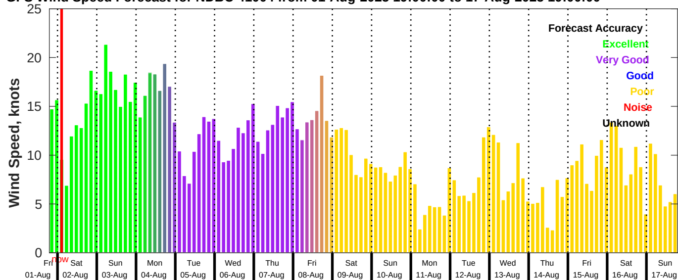
GFS Wind Speed Forecast for NDBC 41004 from 01-Aug-2025 19:00:00 to 17-Aug-2025 19:00:00
