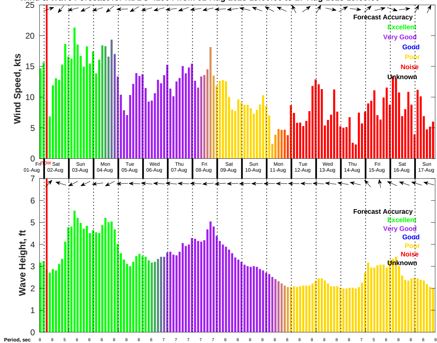
Wind & Wave Forecast for NDBC 41004 from 01-Aug-2025 19:00:00 to 17-Aug-2025 19:00:00
