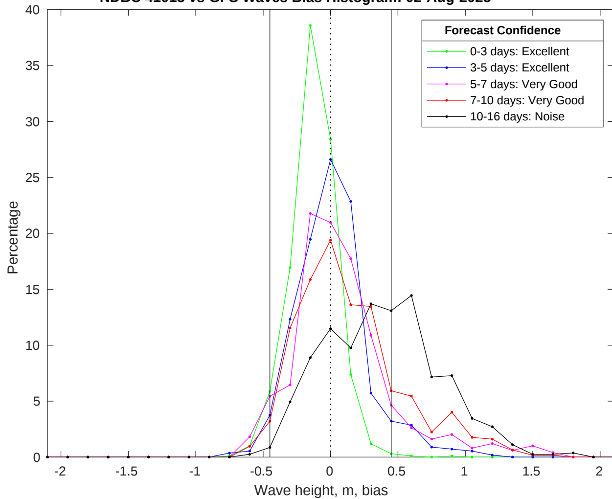
NDBC 41013 vs GFS Waves Bias Histogram: 02-Aug-2025
