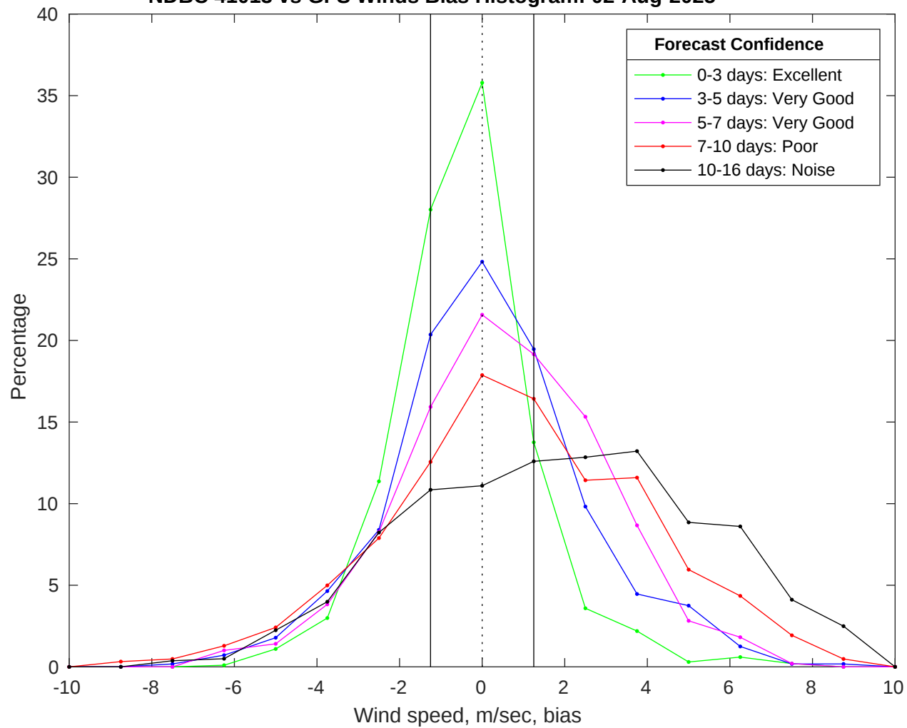
NDBC 41013 vs GFS Winds Bias Histogram: 02-Aug-2025
