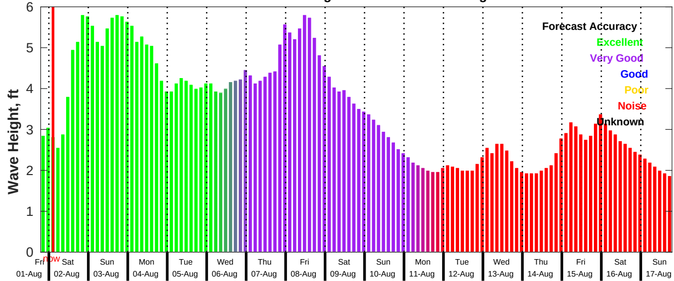
GFS Wave Forecast for NDBC 41013 from 01-Aug-2025 19:00:00 to 17-Aug-2025 19:00:00
