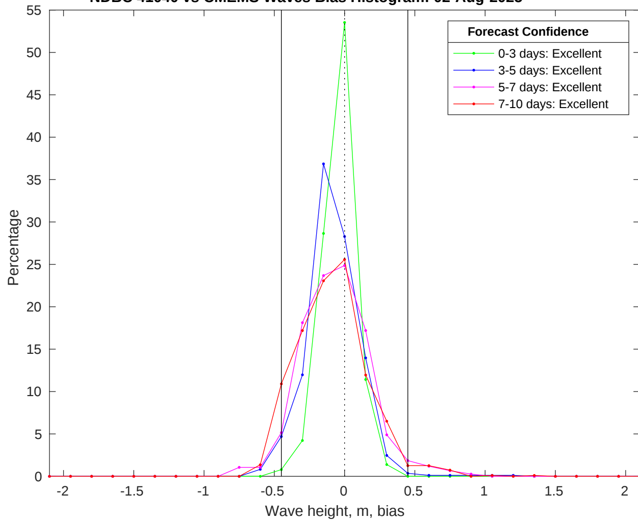
NDBC 41040 vs CMEMS Waves Bias Histogram: 02-Aug-2025
