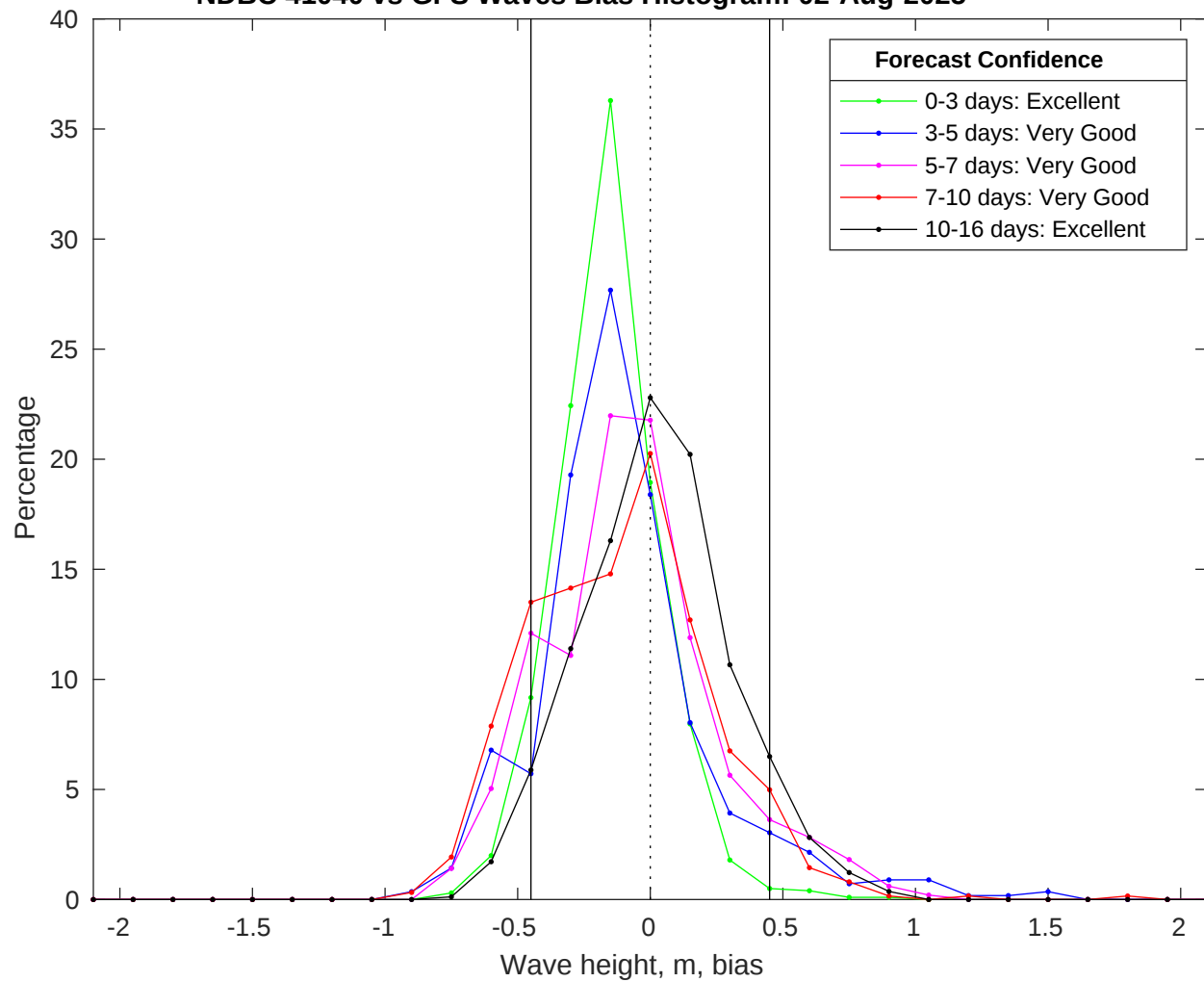
NDBC 41040 vs GFS Waves Bias Histogram: 02-Aug-2025
