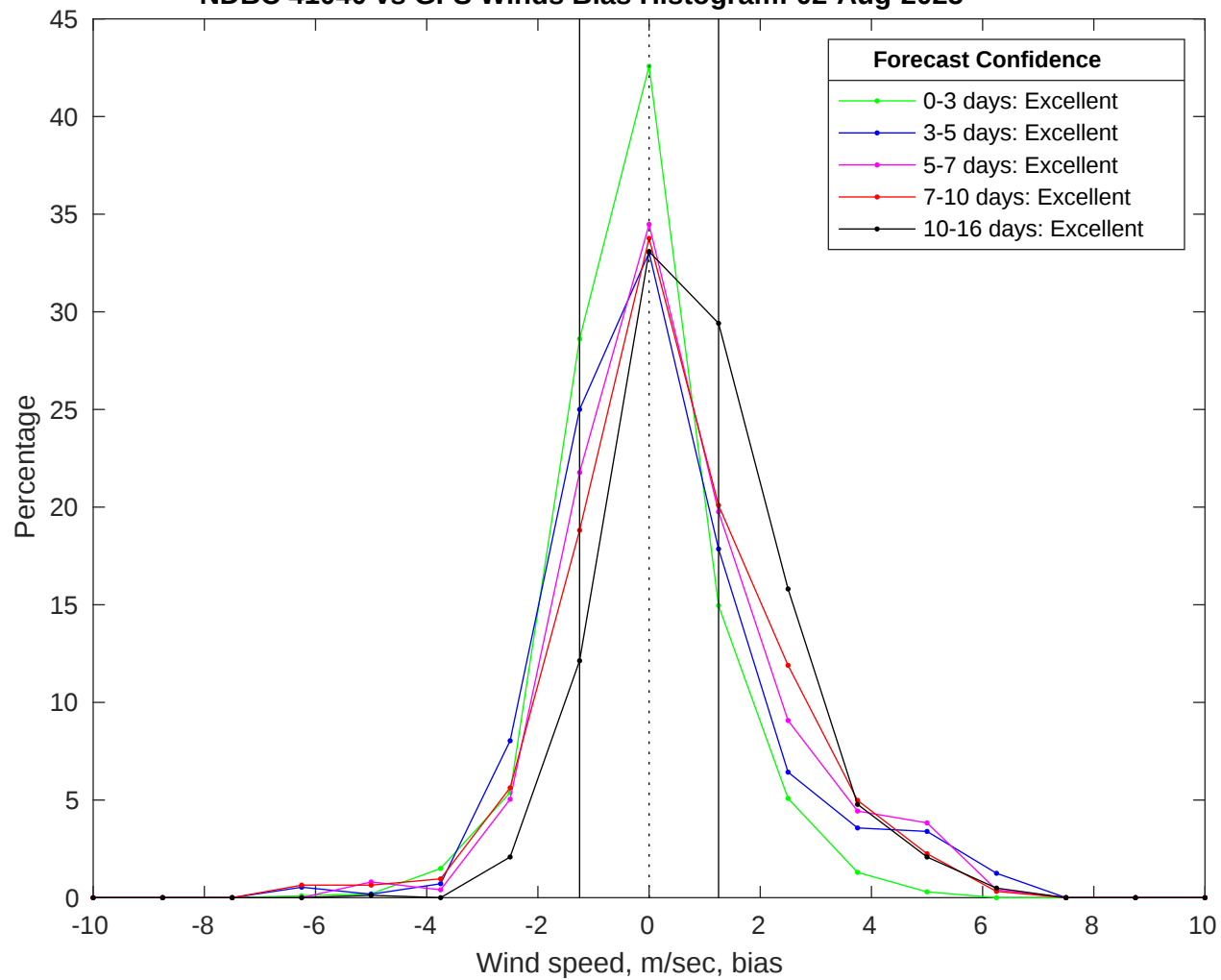
NDBC 41040 vs GFS Winds Bias Histogram: 02-Aug-2025
