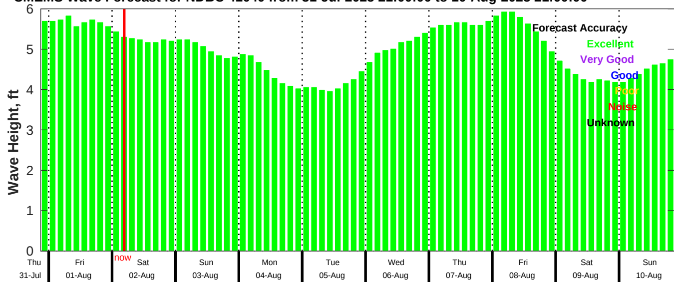
CMEMS Wave Forecast for NDBC 41040 from 31-Jul-2025 21:00:00 to 10-Aug-2025 21:00:00
