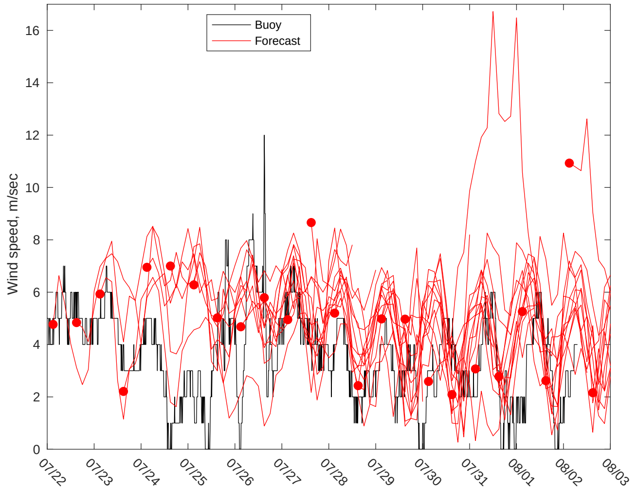
NDBC 42019 vs GFS Winds: 10 to 16 day forecast
