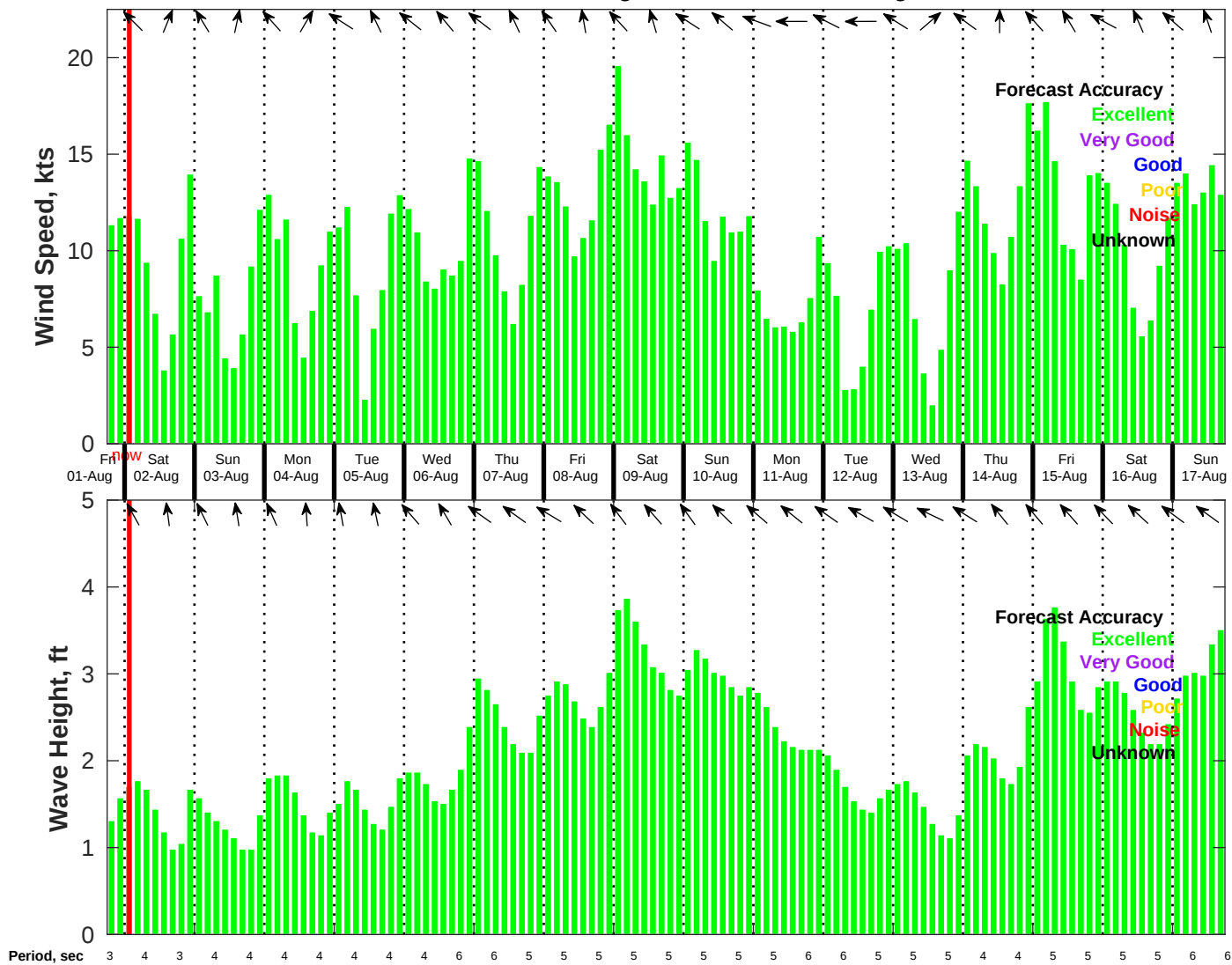
Wind & Wave Forecast for NDBC 42020 from 01-Aug-2025 18:00:00 to 17-Aug-2025 18:00:00
