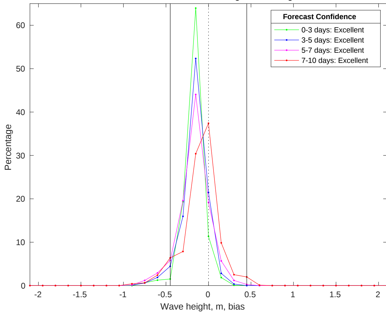
NDBC 42035 vs CMEMS Waves Bias Histogram: 02-Aug-2025
