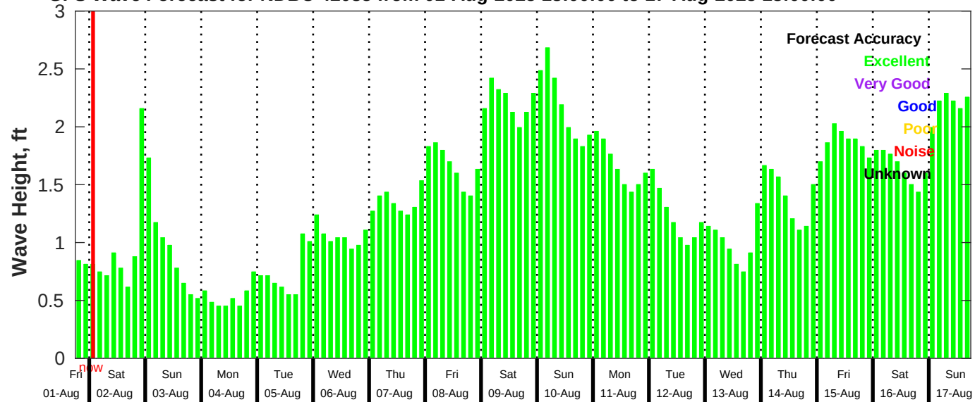
GFS Wave Forecast for NDBC 42035 from 01-Aug-2025 18:00:00 to 17-Aug-2025 18:00:00
