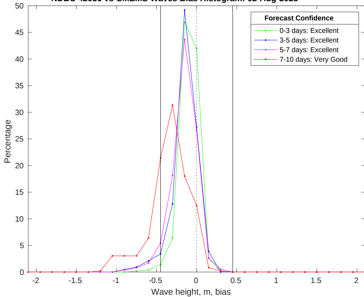
NDBC 42036 vs CMEMS Waves Bias Histogram: 02-Aug-2025
