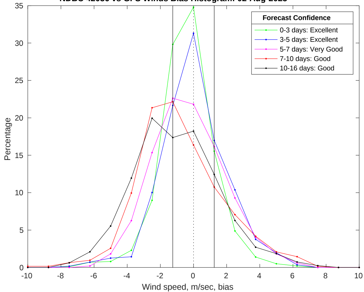
NDBC 42036 vs GFS Winds Bias Histogram: 02-Aug-2025
