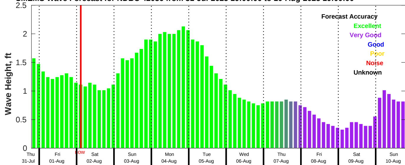
CMEMS Wave Forecast for NDBC 42036 from 31-Jul-2025 19:00:00 to 10-Aug-2025 19:00:00
