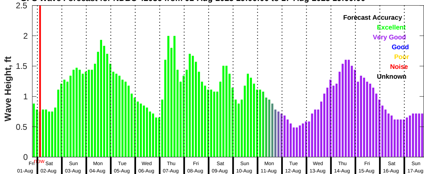
GFS Wave Forecast for NDBC 42036 from 01-Aug-2025 19:00:00 to 17-Aug-2025 19:00:00
