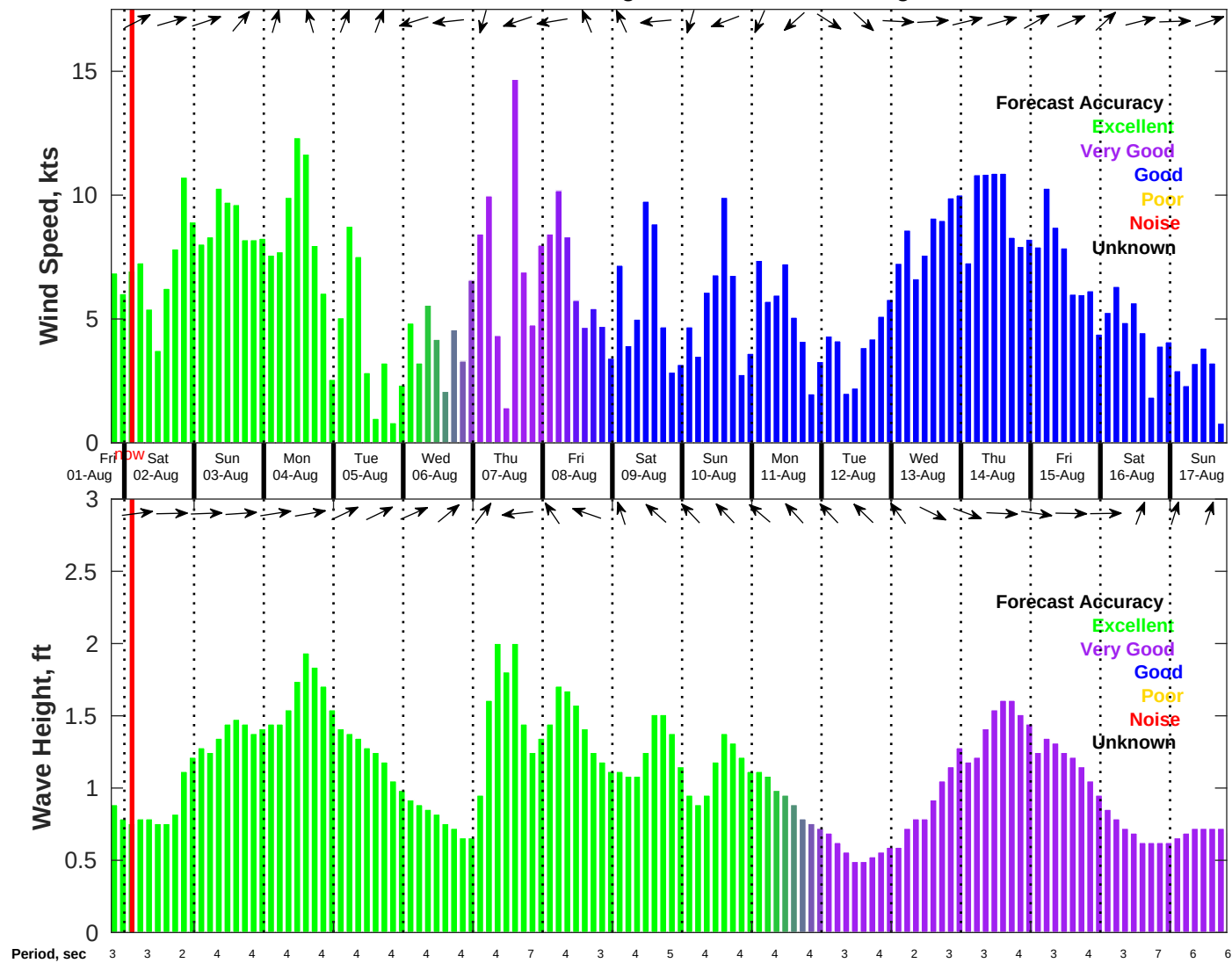
Wind & Wave Forecast for NDBC 42036 from 01-Aug-2025 19:00:00 to 17-Aug-2025 19:00:00
