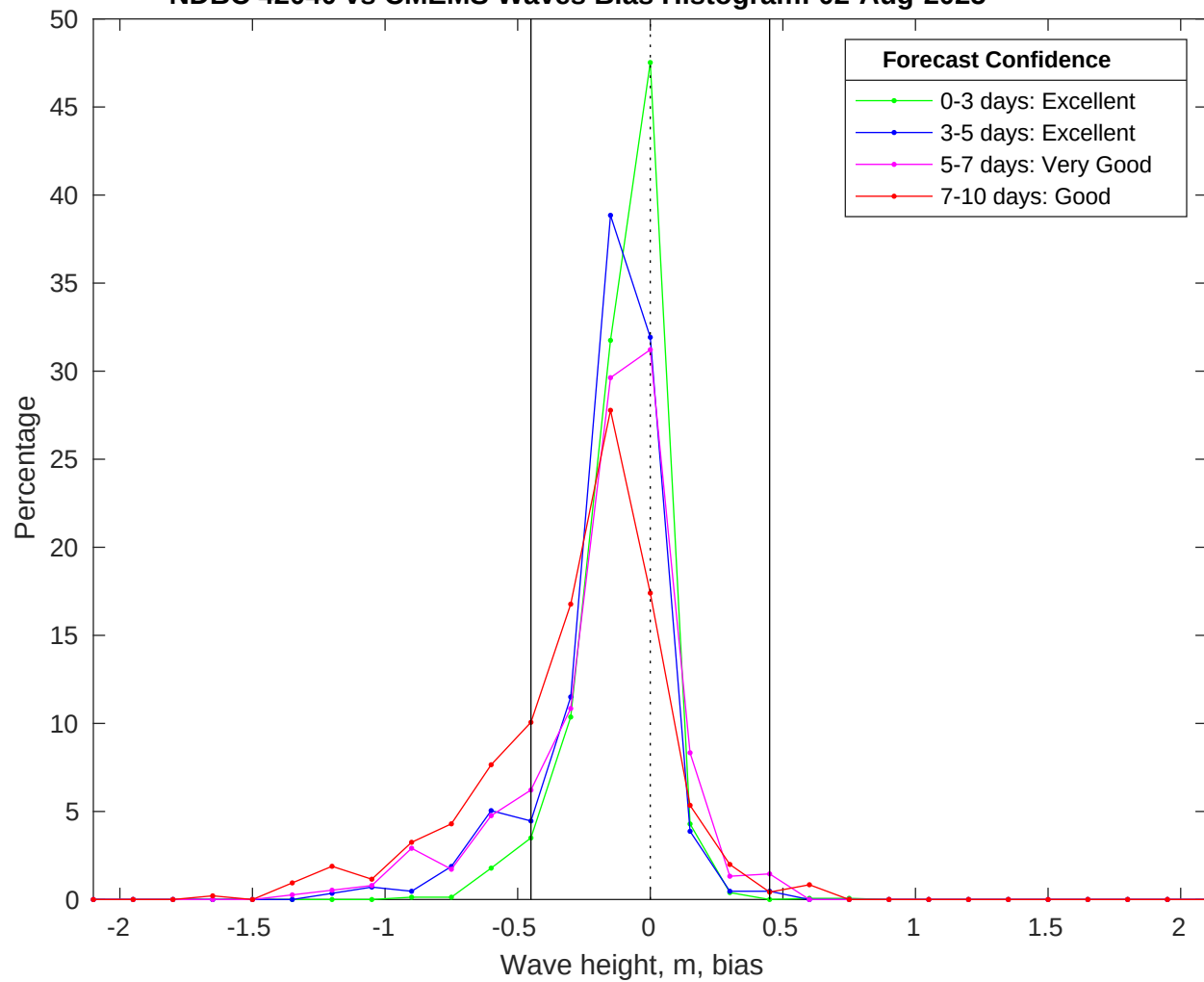
NDBC 42040 vs CMEMS Waves Bias Histogram: 02-Aug-2025
