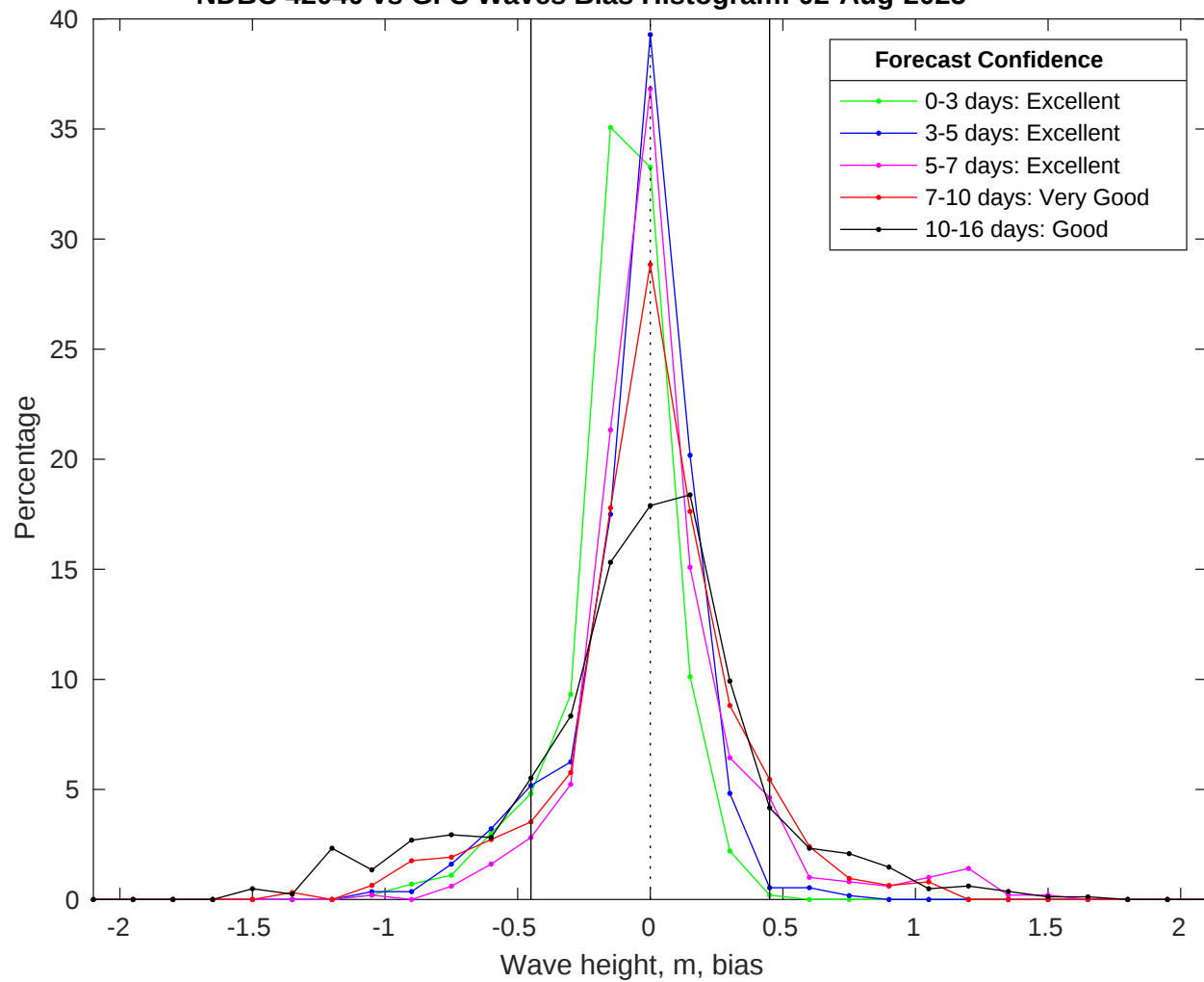
NDBC 42040 vs GFS Waves Bias Histogram: 02-Aug-2025
