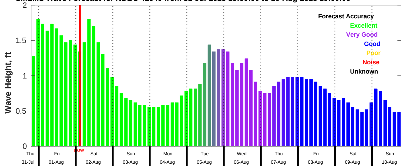
CMEMS Wave Forecast for NDBC 42040 from 31-Jul-2025 19:00:00 to 10-Aug-2025 19:00:00
