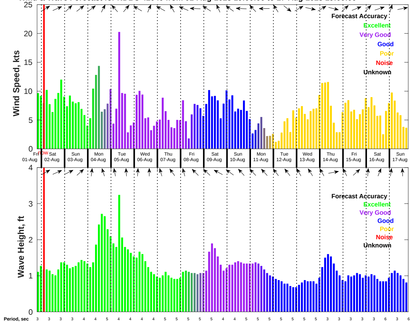
Wind & Wave Forecast for NDBC 42040 from 01-Aug-2025 19:00:00 to 17-Aug-2025 19:00:00
