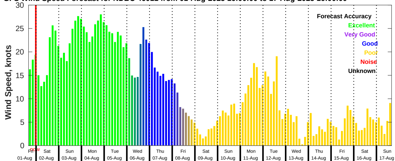
GFS Wind Speed Forecast for NDBC 46011 from 01-Aug-2025 16:00:00 to 17-Aug-2025 16:00:00
