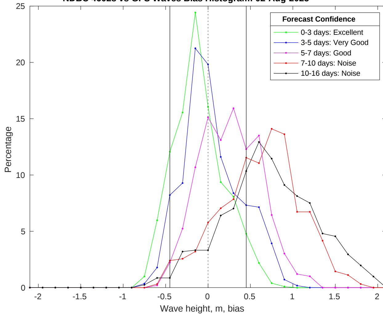
NDBC 46028 vs GFS Waves Bias Histogram: 02-Aug-2025
