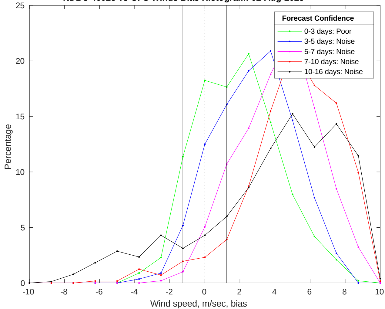
NDBC 46028 vs GFS Winds Bias Histogram: 02-Aug-2025
