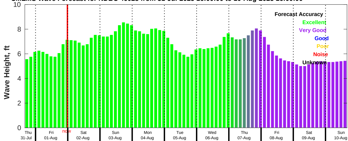
CMEMS Wave Forecast for NDBC 46028 from 31-Jul-2025 16:00:00 to 10-Aug-2025 16:00:00
