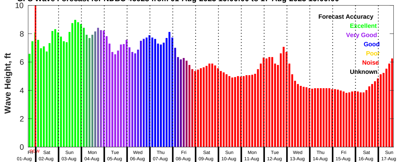
GFS Wave Forecast for NDBC 46028 from 01-Aug-2025 16:00:00 to 17-Aug-2025 16:00:00
