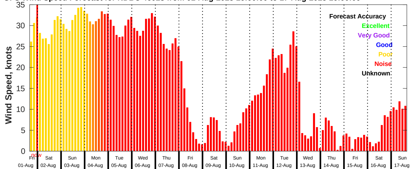
GFS Wind Speed Forecast for NDBC 46028 from 01-Aug-2025 16:00:00 to 17-Aug-2025 16:00:00
