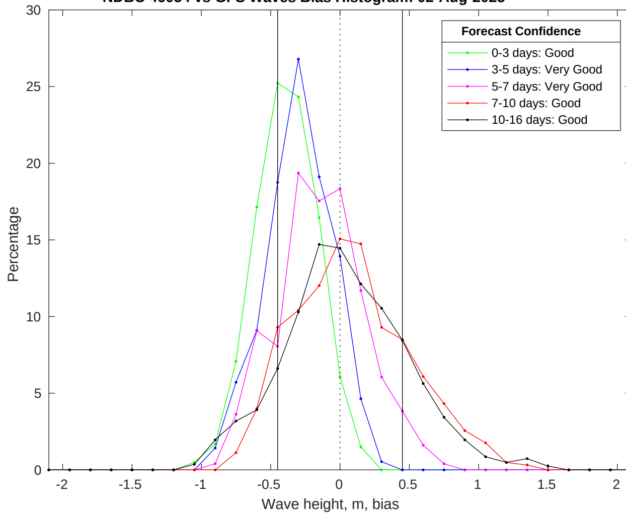
NDBC 46054 vs GFS Waves Bias Histogram: 02-Aug-2025
