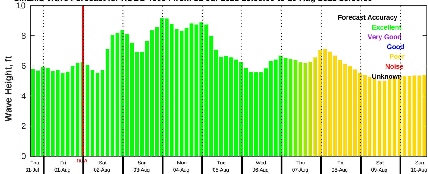
CMEMS Wave Forecast for NDBC 46054 from 31-Jul-2025 16:00:00 to 10-Aug-2025 16:00:00
