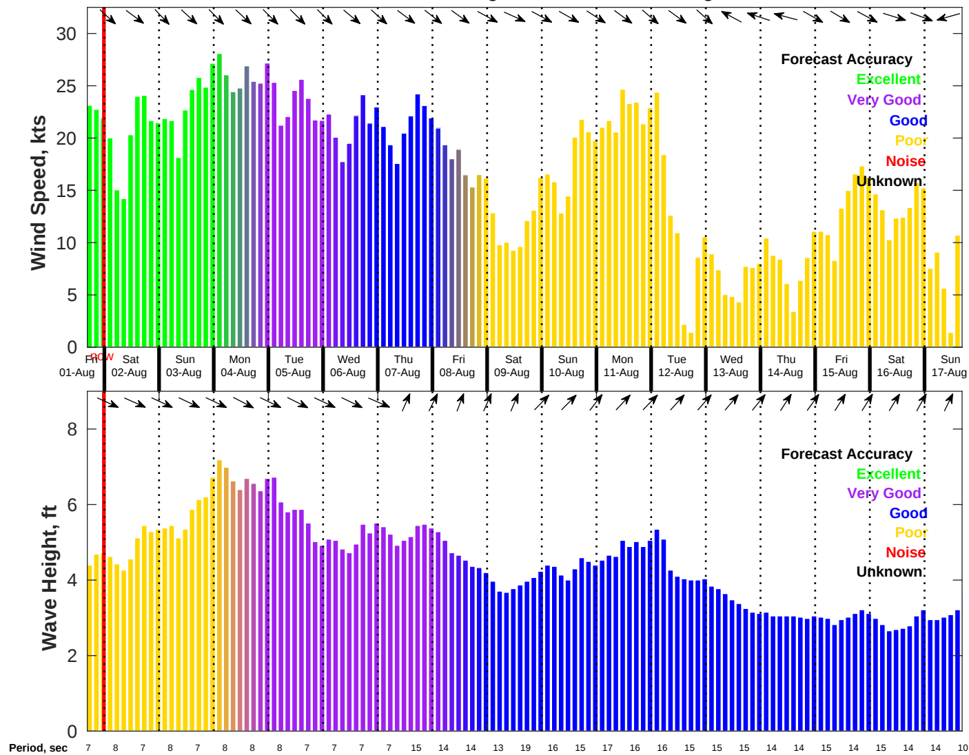
Wind & Wave Forecast for NDBC 46054 from 01-Aug-2025 16:00:00 to 17-Aug-2025 16:00:00
