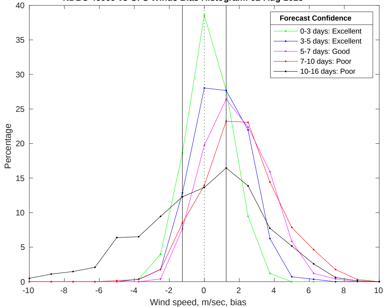
NDBC 46069 vs GFS Winds Bias Histogram: 02-Aug-2025
