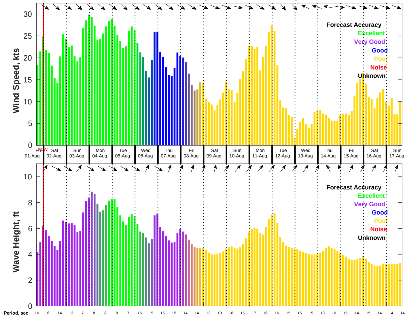
Wind & Wave Forecast for NDBC 46069 from 01-Aug-2025 16:00:00 to 17-Aug-2025 16:00:00
