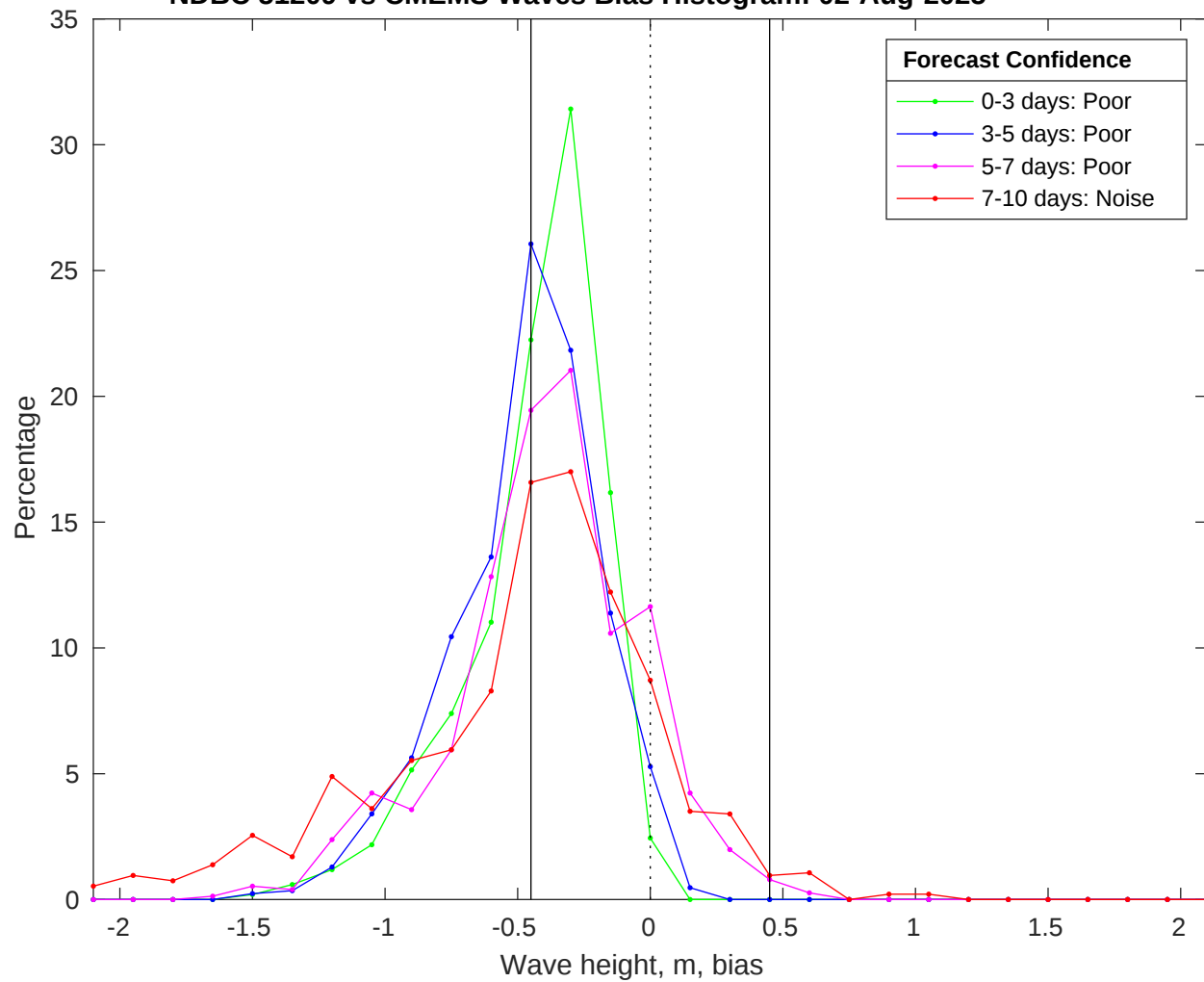
NDBC 51209 vs CMEMS Waves Bias Histogram: 02-Aug-2025
