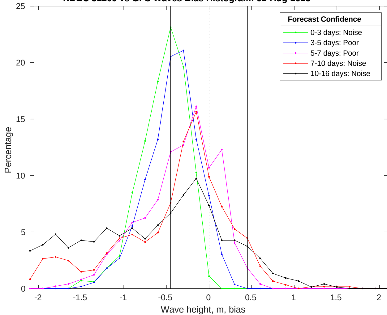
NDBC 51209 vs GFS Waves Bias Histogram: 02-Aug-2025
