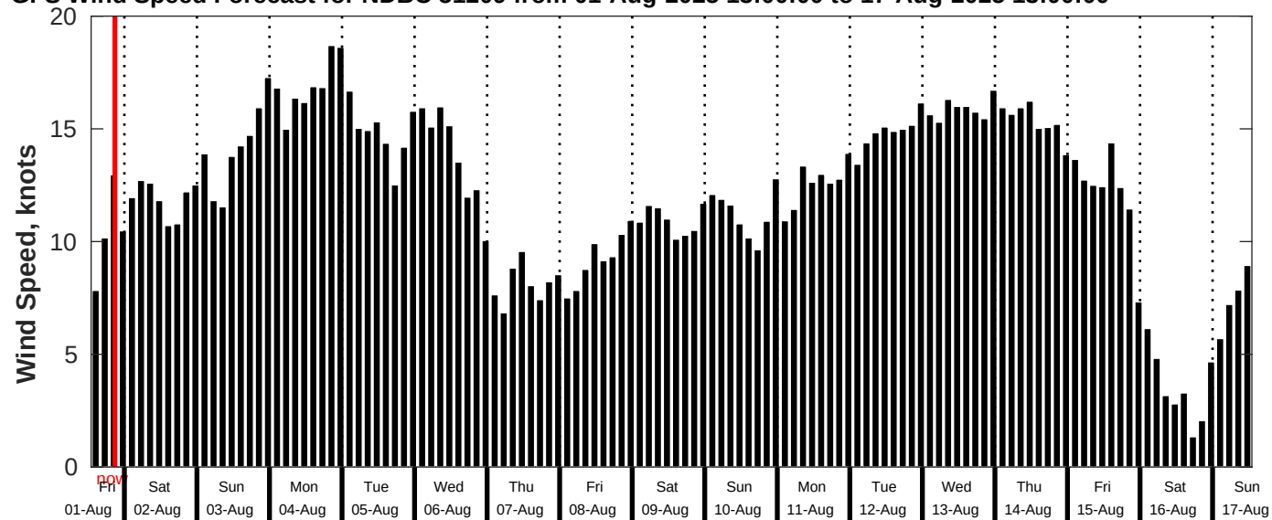
GFS Wind Speed Forecast for NDBC 51209 from 01-Aug-2025 13:00:00 to 17-Aug-2025 13:00:00
