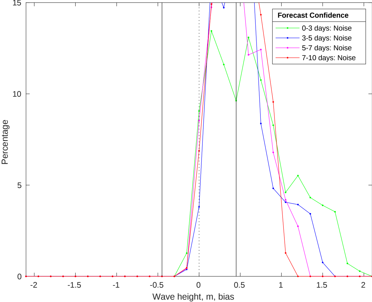
NDBC 51211 vs CMEMS Waves Bias Histogram: 02-Aug-2025
