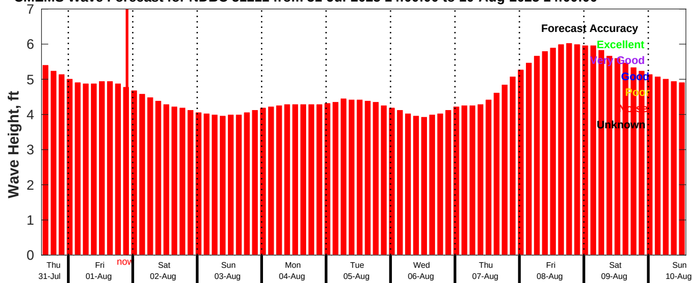
CMEMS Wave Forecast for NDBC 51211 from 31-Jul-2025 14:00:00 to 10-Aug-2025 14:00:00
