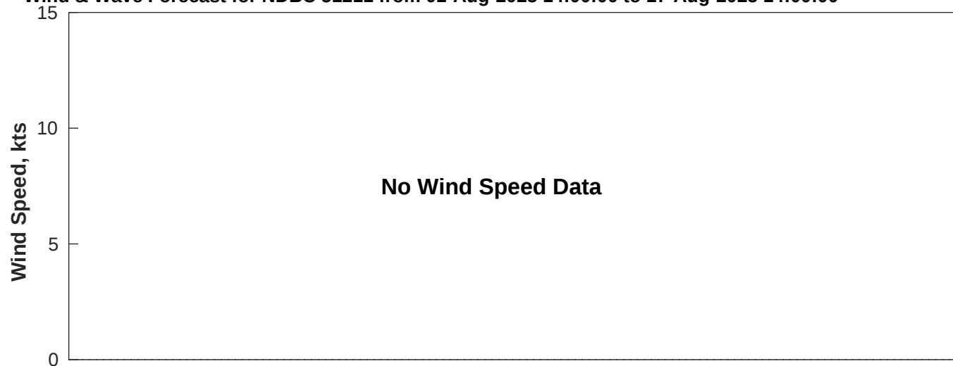
Wind & Wave Forecast for NDBC 51211 from 01-Aug-2025 14:00:00 to 17-Aug-2025 14:00:00
